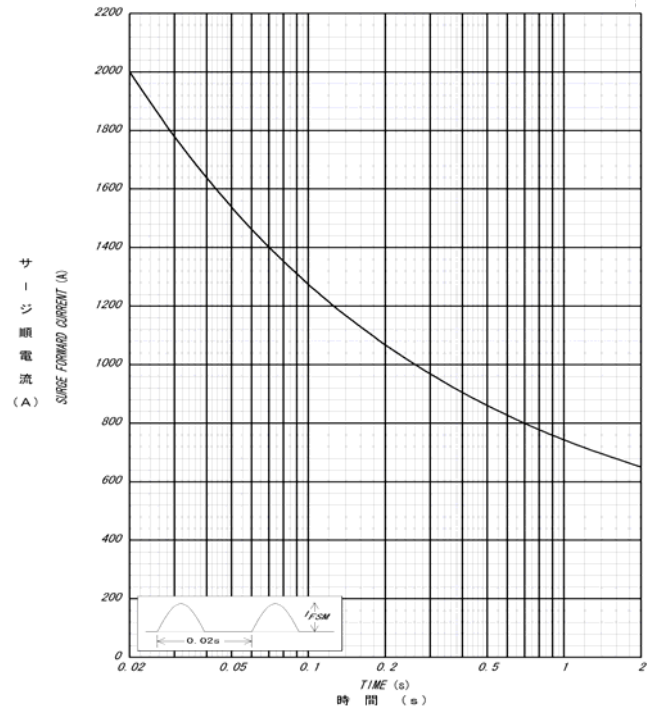
サージ順電流定格 SURGE CURRENT RATINGS f=50Hz, Half Sine Wave, Non-Repetitive, Tj=125°C
